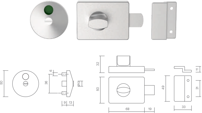
P5020 Premium Indicator Set SC
