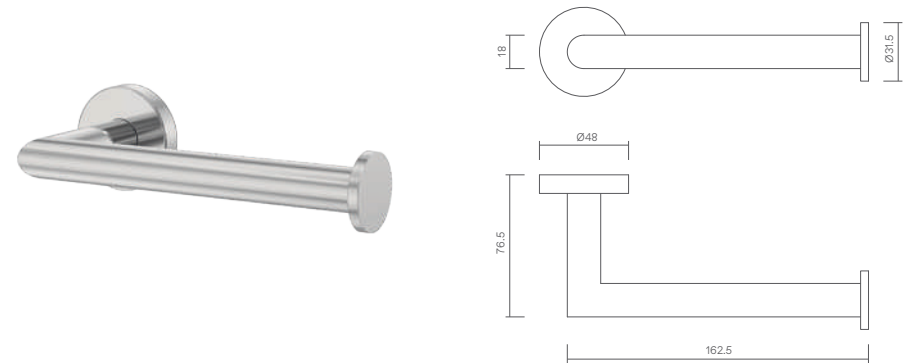
P0740 Dual Fix Single Bar Toilet Roll Holder PSS
