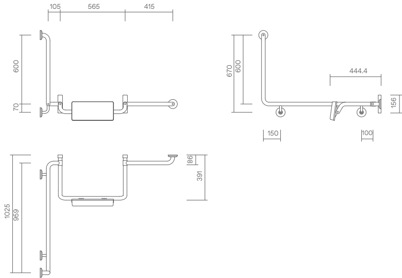
P0938 - RH Version Pictured
