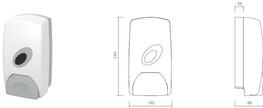
P0102 Refillable Soap Dispenser ABS Plastic
