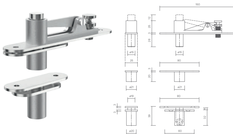
J1002SSS Heavy Duty Pivot Set 200kg SSS
