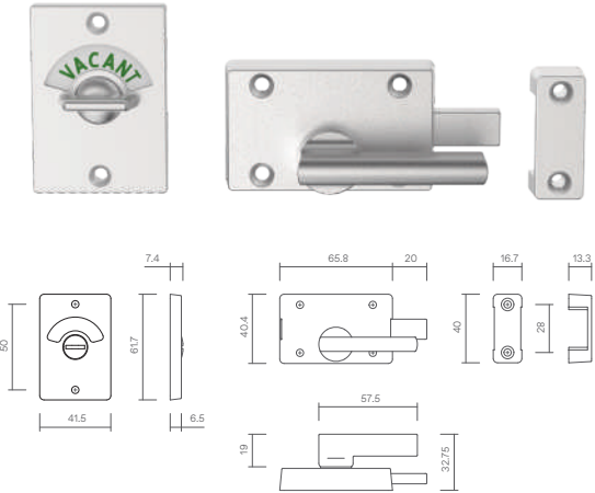
P5033SC Disabled Compliant Screw Indicator Set SC P5033BLK Disabled Compliant Screw Indicator Set BLK
