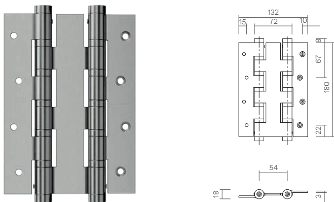
J4100SSS Double Action Hinge 50kg 180×132×3mm SSS
