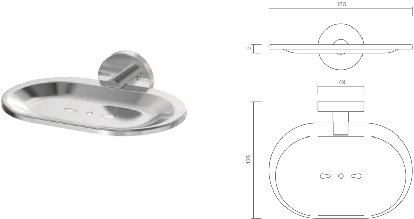
P0745 Dual Fix Soap Dish PSS ✓
