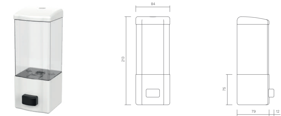
P0101 Refillable Soap Dispenser ABS Plastic
